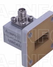
62WCA3.5 Right Angle Rectangular Waveguide to Coaxial Adapter 12.4-18GHz WR62 to 3.5mm Female
