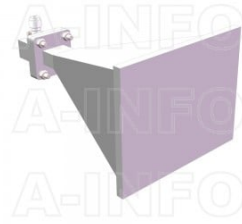
LB-62-20-C-TFSPO Standard Gain Horn Antenna 12.4-18GHz 20dB Gain TNC Female
