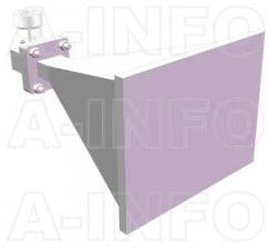
LB-62-20-C-7SPO Standard Gain Horn Antenna 12.4-18GHz 20dB Gain 7mm
